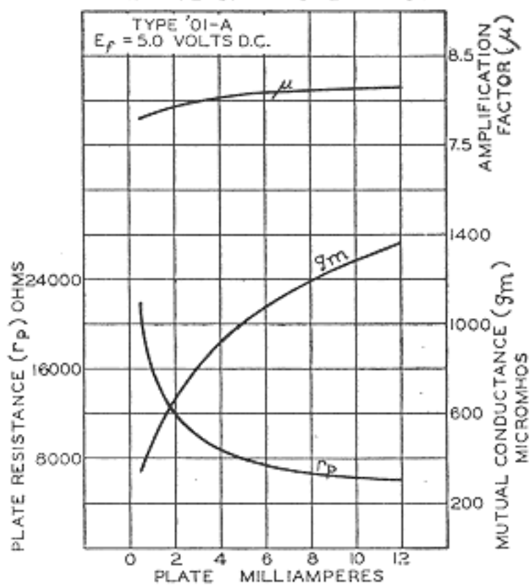
AVERAGE CHARACTERISTICS
